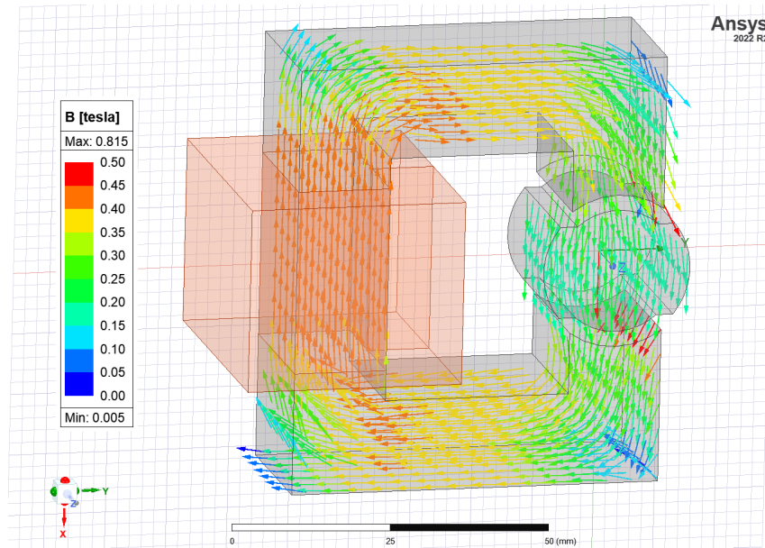
Figure 15: Flux density at 90° for non-linear material in 3D FEA
