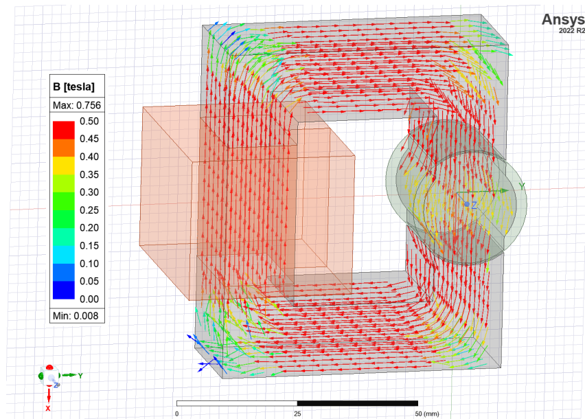
Figure 13: Flux density at 0° for non-linear material in 3D FEA
