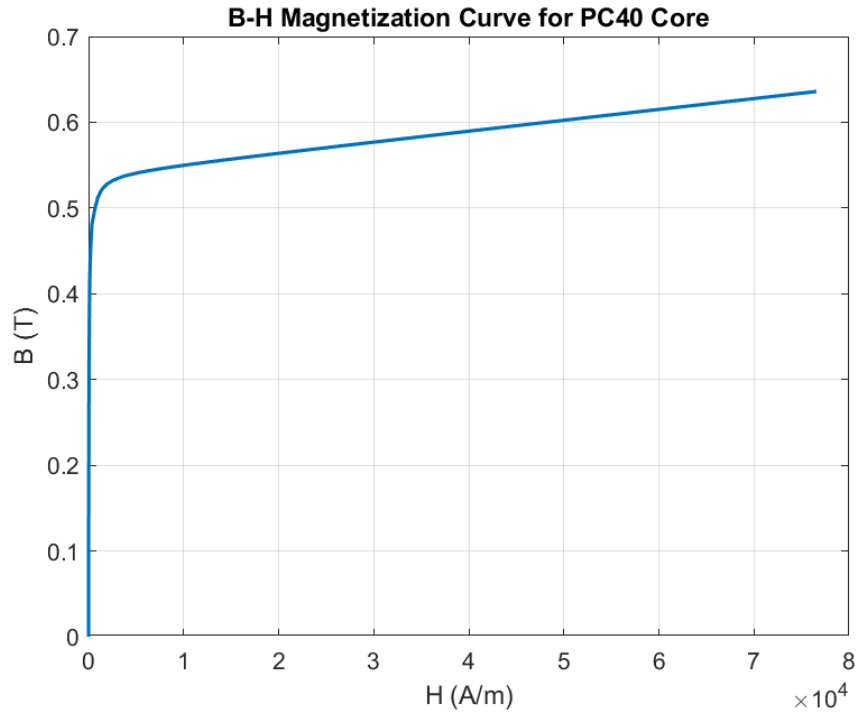
Figure 17: B-H curve of the PC40 core used in the FEA simulations.
