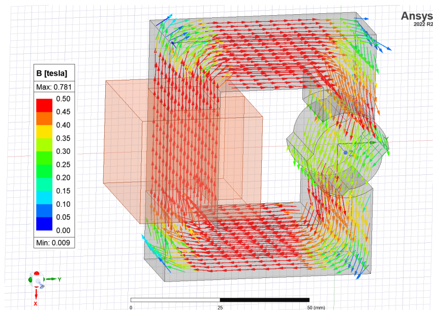
Figure 14: Flux density at 45° for non-linear material in 3D FEA
